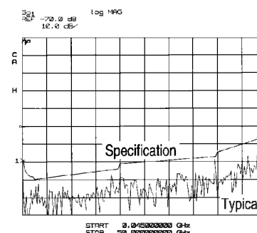
System dynamic range
