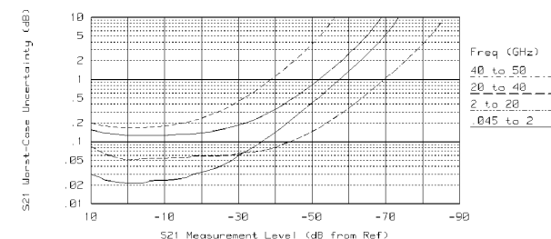
Measurement port characteristics Magnitude
